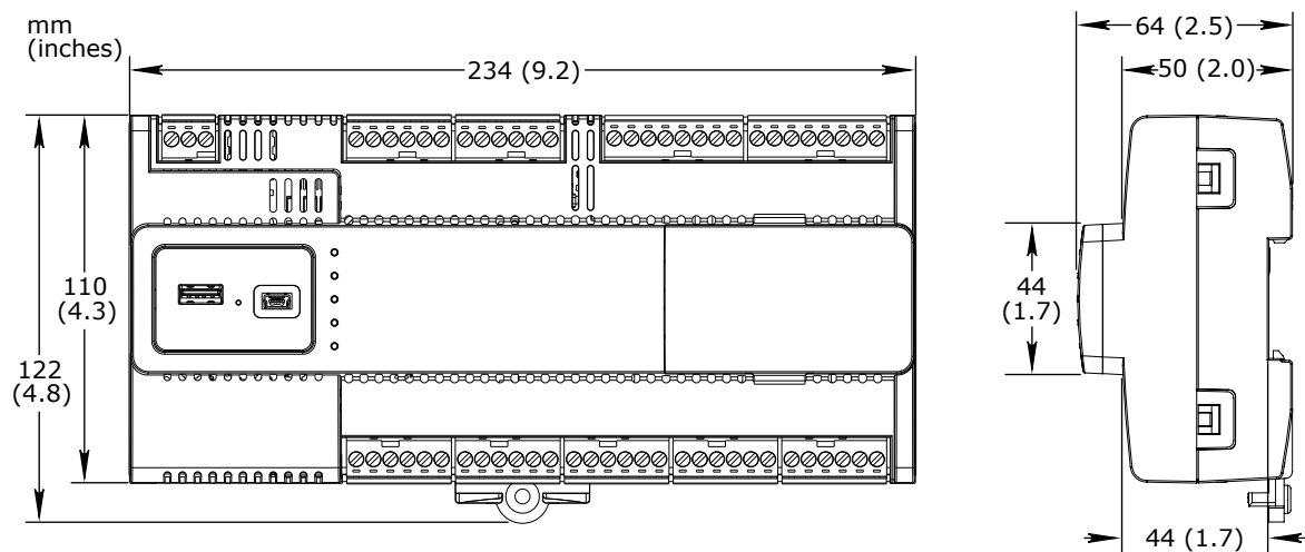
Dimensions (MP-C-24A, -36A) 234 W x 110 H x 64 D mm (9.2 W x 4.3 H x 2.5 D in.)
